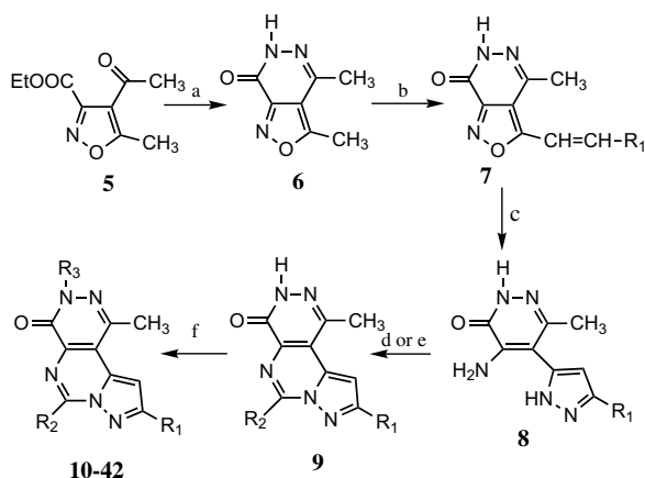
Scheme 1. Reagents and conditions: (a) hydrazine hydrate, EtOH, rt; (b) R 1 CHO, MeONa, abs MeOH, reflux; (c) hydrazine hydrate, EtOH, rt; (d) (R 2 CO) 2 O, reflux; (e) R 2 COOH, dichloromethane, anhydrous DMF, DMAP, EDC, reflux; (f) R 3 X, NaH, DMSO, rt.
